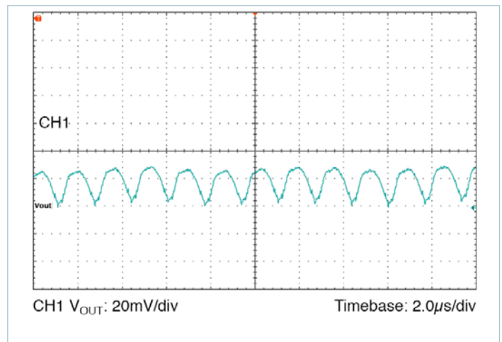
Figure 52 — Output voltage ripple: nominal line, nominal trim, 50% load, C OUT = 12 x 47μF ceramic
