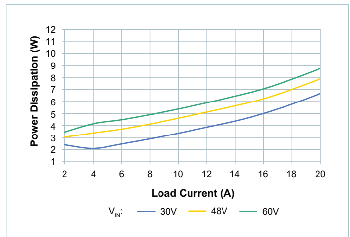
Figure 47 — System power dissipation, high trim, board temperature = -40°C
