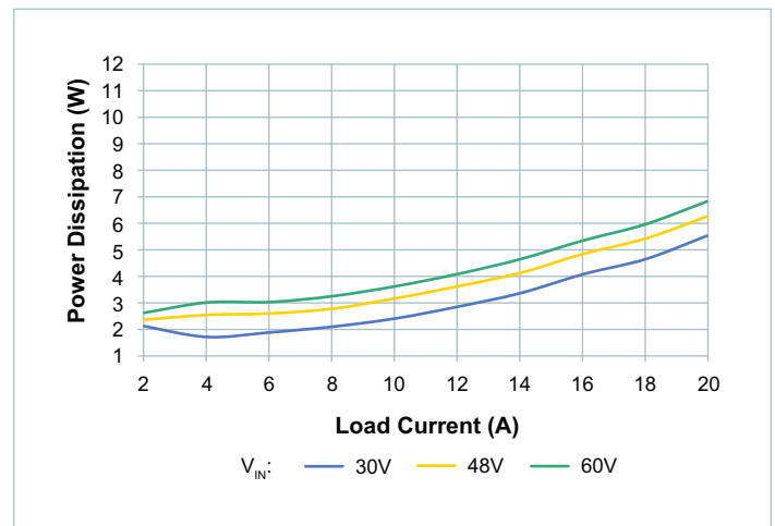
Figure 46 — System power dissipation, low trim, board temperature = -40°C
