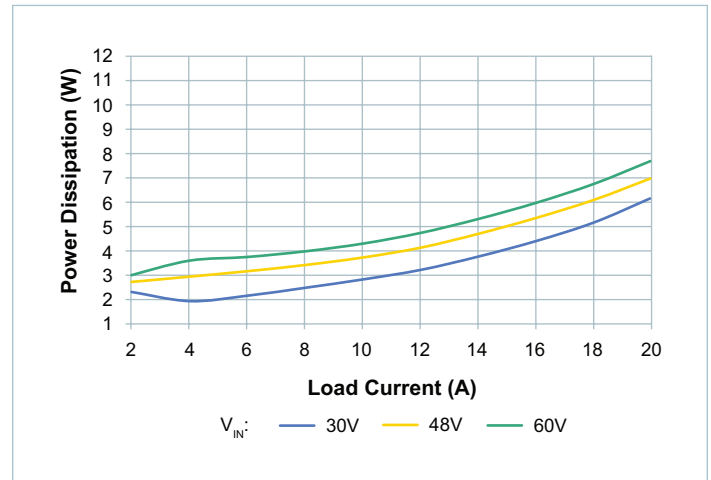
Figure 45 — System power dissipation, nominal trim, board temperature = -40°C
