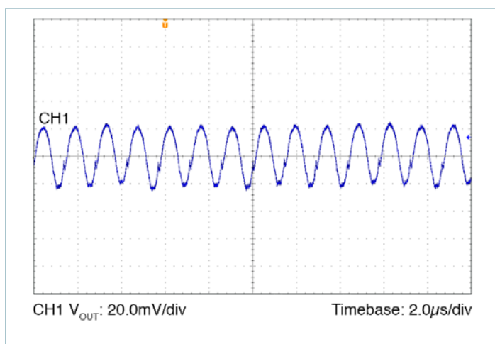
Figure 77 — Output voltage ripple: nominal line, nominal trim, 50% load, C OUT = 6 x 47µF ceramic, 20MHz BW
