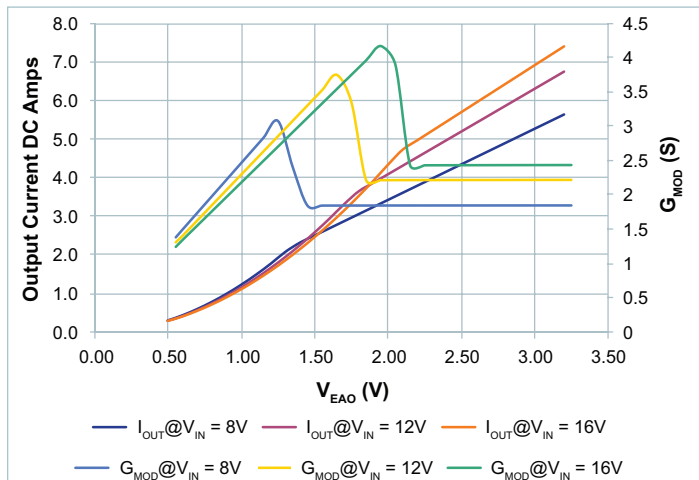
Figure 69 — G_{MOD} vs output current vs. V_{EAO} , V_{OUT} = 12V ; 8 – 16 V_{IN}
