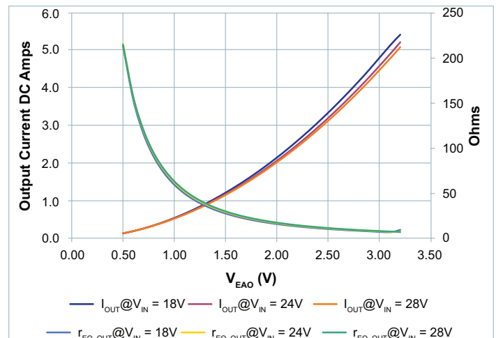
Figure 91 — r_{EQ\_OUT} vs. output current vs. V_{EAO} , V_{OUT} = 28\text{V} ; 18 – 28 V_{IN}
