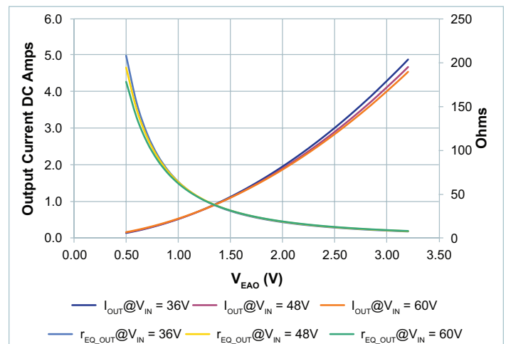
Figure 92 — r_{EQ\_OUT} vs. output current vs. V_{EAO} , V_{OUT} = 28\text{V} ; 36 – 60 V_{IN}
