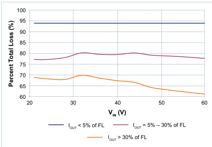
Figure 41 — V_{OUT} = 40V
