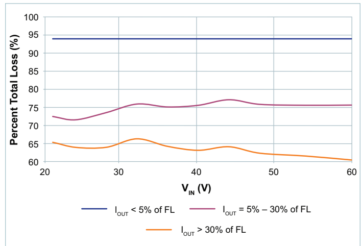
Figure 44 — V_{OUT} = 50V
