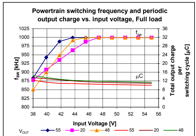
Figure 14 – Powertrain switching frequency and periodic output charge vs. V_{IN} , V_{OUT} ; I_{OUT}=12.5A
