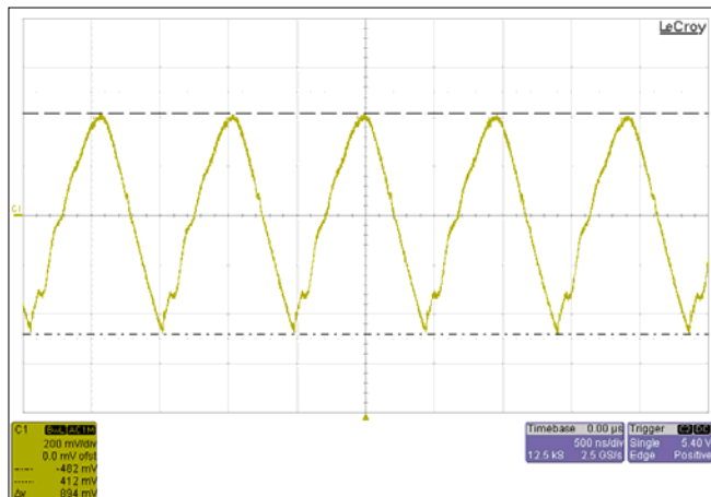
Figure 13 – Typical output voltage ripple waveform, T_{CASE} = 30^{\circ}C , V_{IN}=45V , V_{OUT}=48V , I_{OUT}=12.5A , no external capacitance.
