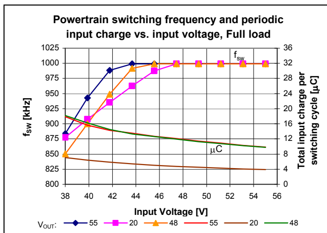
Figure 15 – Powertrain switching frequency and periodic input charge vs. V_{IN} , V_{OUT} ; I_{OUT}=12.5A
