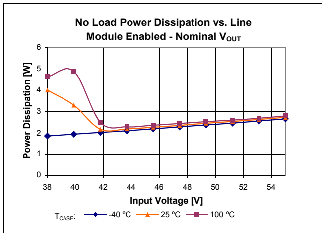
Figure 1 - No load power dissipation vs. V_{IN} , module enabled
