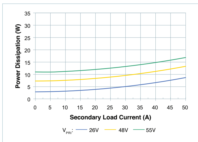
Figure 4 — Power dissipation at -40^\circ\text{C}
