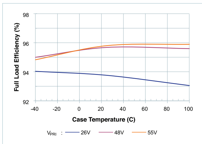
Figure 2 — Full secondary load efficiency vs. temperature
