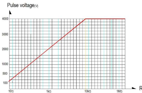
Pulse load rating in accordance with IEC 60115-1,4.27; 1.2µs/50µs ; 5 pulses loaded, for permissible resistance change <\pm(0.5\%+0.05\Omega)
