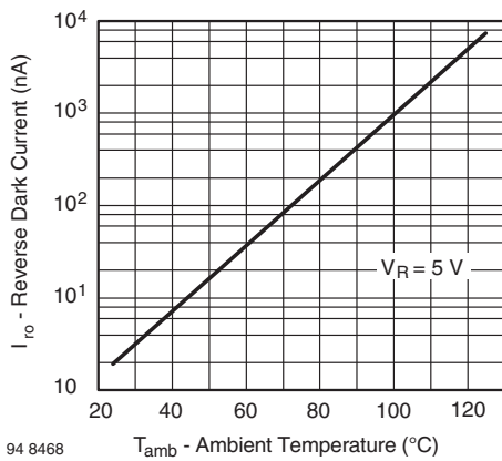
94 8468 T_{amb} - Ambient Temperature ( ^{\circ}\text{C} ) Fig. 1 - Reverse Dark Current vs. Ambient Temperature
