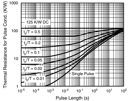
Fig. 7 - Thermal Response
