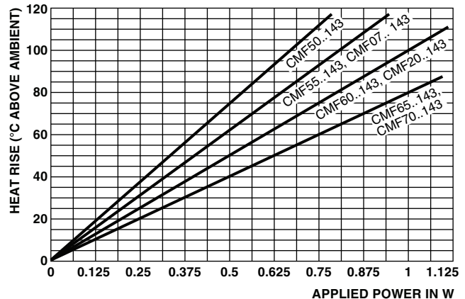
THERMAL RESISTANCE
