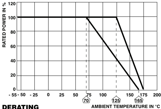
DERATING
