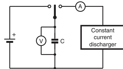
Fig. 14 - Test Circuit for Capacitance Measurement
