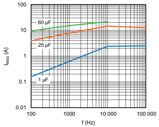
Maximum RMS current as function of frequency T_{amb} \leq 85\text{ }^{\circ}\text{C} ; U_r = 250\text{ V}_{AC}
