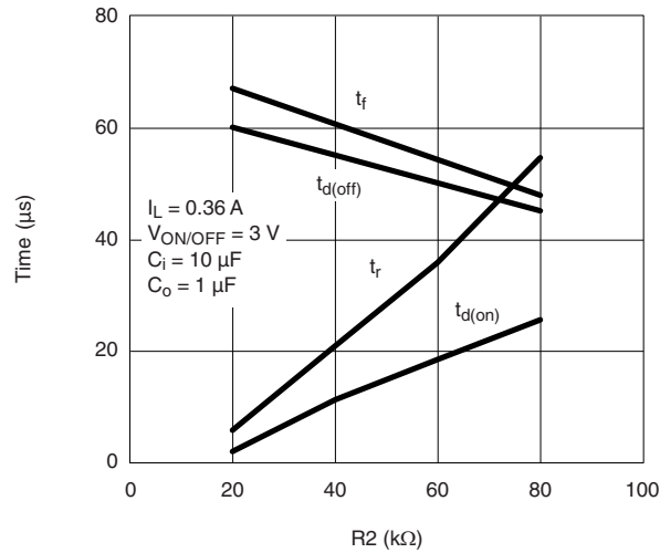
Switching Variation R2 at V_{IN} = 1.8 \text{ V} , R1 = 300 k\Omega
