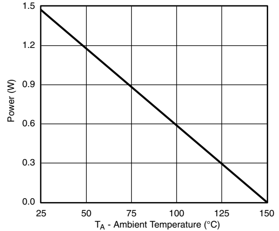
Power Derating
