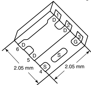
PowerPAK SC-70-6L-Single
