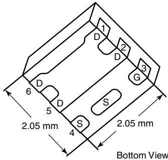
PowerPAK SC-70-6L-Single
