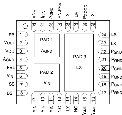
SiC403A/B Pin Configuration (Top View)
