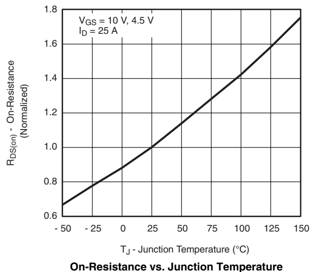
V_{GS} = 10\text{ V, }4.5\text{ V} I_D = 25\text{ A} On-Resistance vs. Junction Temperature
