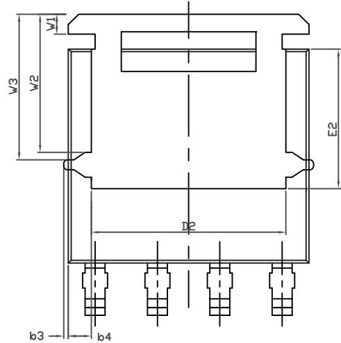
BACKSIDE VIEW(SINGLE)
