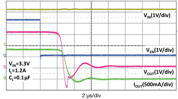
Fig. 36 - Enable Power Down
