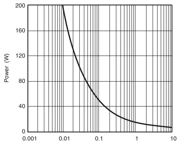
Power (W) Single Pulse Power, Junction-to-Ambient
