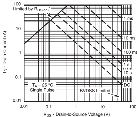
T_A = 25\text{ }^\circ\text{C} Single Pulse BVDSS Limited Safe Operating Area, Junction-to-Ambient
