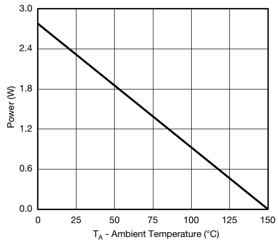
Power, Junction-to-Ambient
