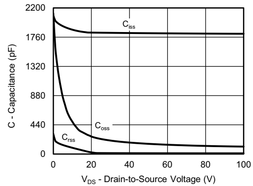
Capacitance
