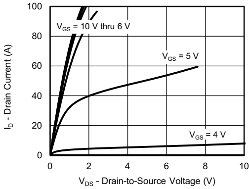
Output Characteristics
