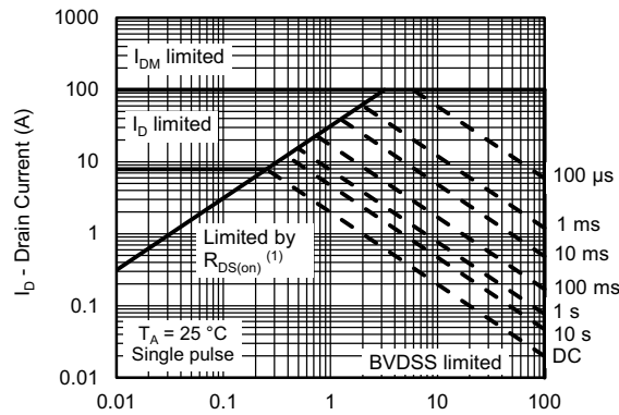
Safe Operating Area, Junction-to-Ambient
