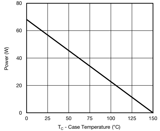
Power, Junction-to-Case
