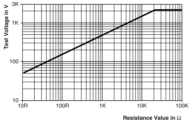
10 / 700 Pulse
