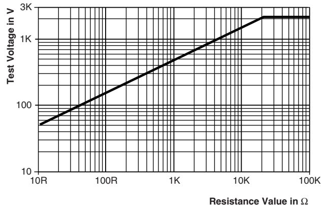
10 / 700 Pulse
