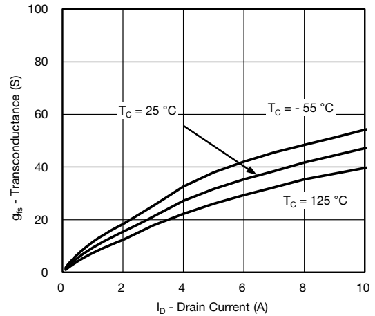
Transconductance
