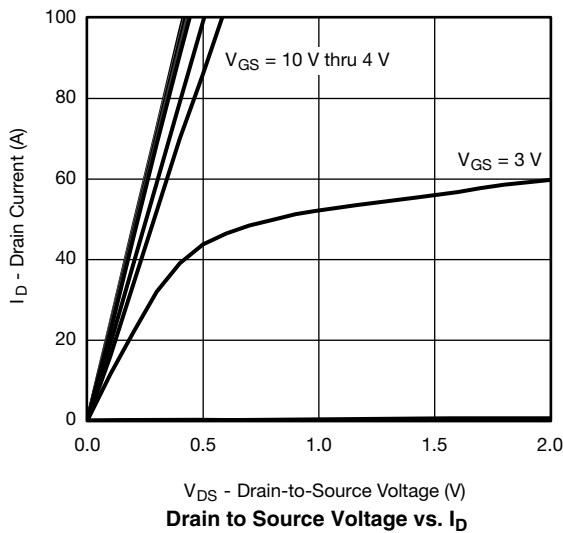
Drain to Source Voltage vs. I_D
