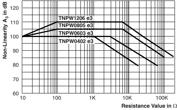
Non-Linearity
