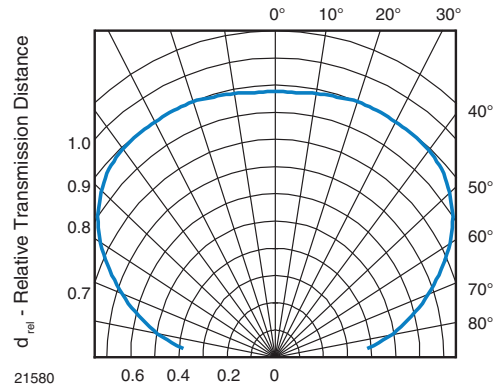
Fig. 12 - Vertical Directivity
