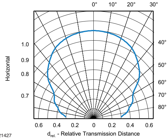
Fig. 11 - Horizontal Directivity
