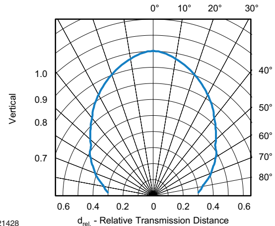
Fig. 12 - Vertical Directivity
