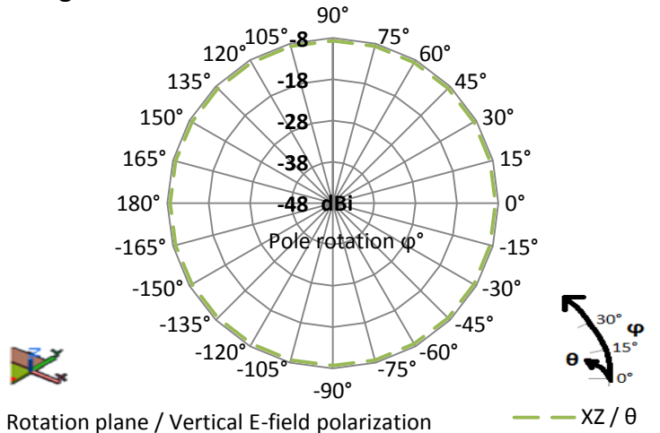
Figure 6 VJ5301M400MXBSR XZ Radiation Pattern
