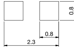
Recommended solder pad footprint
