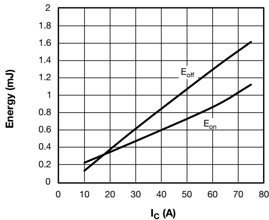
Fig. 7 - Typical Q1 - Q4 Trench IGBT Energy Loss vs. I_C (with D5 - D6 Clamping Diode) T_J = 125\text{ }^\circ\text{C} , V_{CC} = 300\text{ V} , R_g = 4.7\text{ }\Omega , V_{GE} = 15\text{ V} , L = 500\text{ }\mu\text{H}
