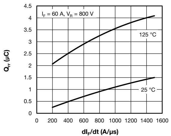
Fig. 8 - Diode Reverse Recovery Charge vs. dl_F/dt
