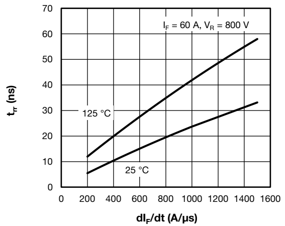
Fig. 7 - Diode Reverse Recovery Current vs. dl_F/dt
