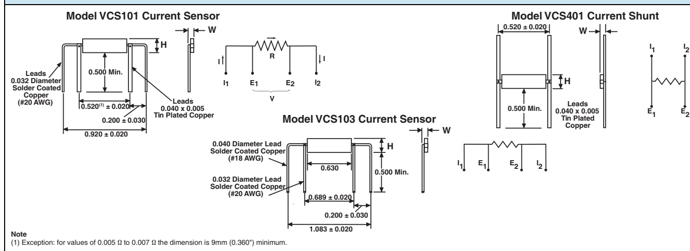
FIGURE 1 - DIMENSIONS AND SCHEMATIC
