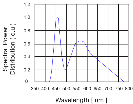
Fig 5. Spectral Power Distribution
