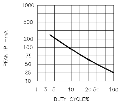
PEAK I P —mA DUTY CYCLE% Fig.6 MAX PEAK CURRENT VS. DUTY CYCLE % (REFRESH RATE f=1KHz)
