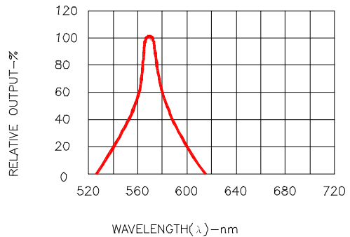
RELATIVE OUTPUT—% WAVELENGTH(λ)—nm Fig.2 SPECTRAL RESPONSE
