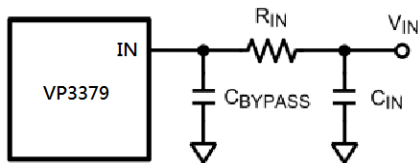
Figure 7 Reducing IC Input Noise
