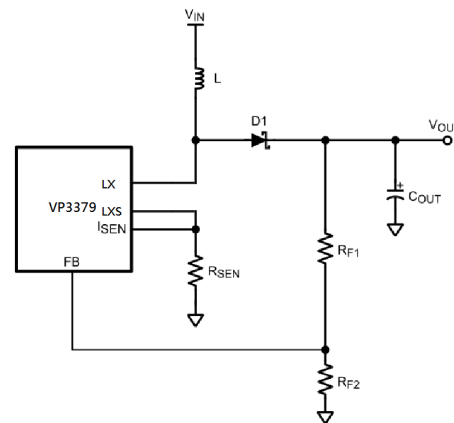
Figure 6. Adjusting the Output Voltage
