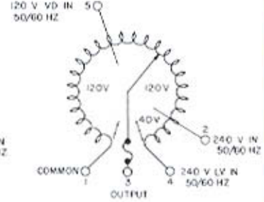
6020 Ganged Unit
