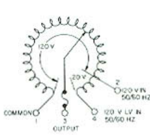
6011 Ganged Unit
