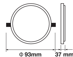
Cutting Size: \varnothing 72 mm
