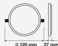
Cutting Size: \varnothing 95 mm
