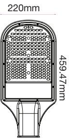
STREETLIGHT-ADAPTER
