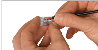
Strip conductor to 11 mm.
