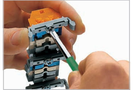
Terminal strip with fixing flanges, screw mounting of 209-123 mounting adapter (The distance between mounting adapters should be 25 - 30 mm).
