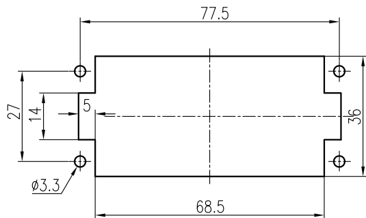
面板安装开孔图 Panel cut out
