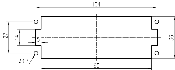
面板安装开孔图 Panel cut out
