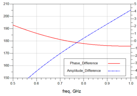
Amplitude and Phase Balance
