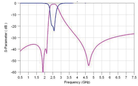
RFBPF2012090AS1T35
