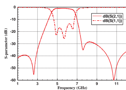
RFBPF1608060K788Q1C
