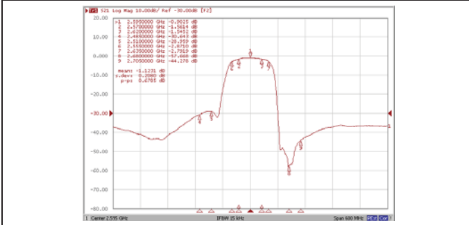
SF11092350B4005T
