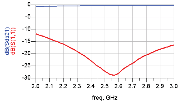
RFBLN10052G5W37N2T
