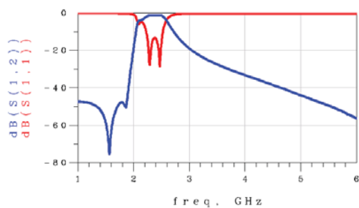
RFBPF1608060K68Q1C
