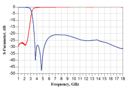
RFLPF1608060AAT
