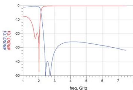
RFLPF1005040A1T
