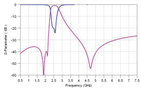
RFBPF2012040AHT
