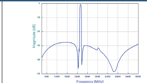
SF14112350B4001T
