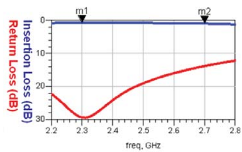
Insertion and Return Loss
