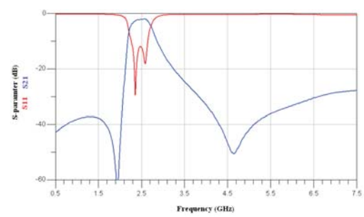
RFBPF2012080AFT
