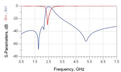
RFBPF2012040AHT
